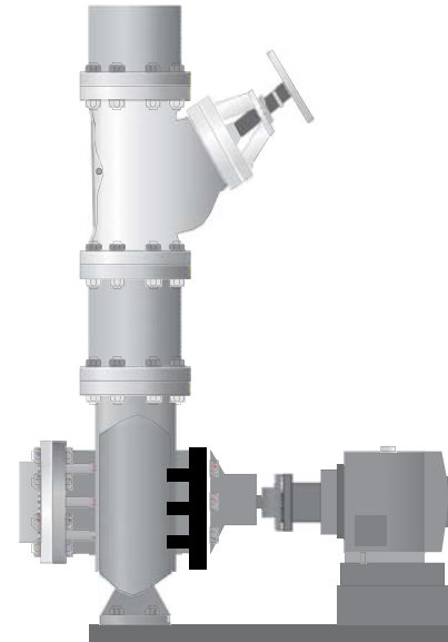
Figure 2: Illustration of Installed Model TDV Valve with Pump
