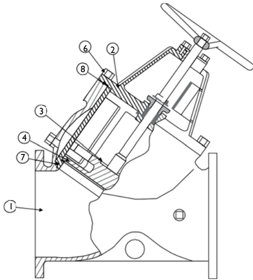
Figure 4: Illustration of Model TDV Valve
