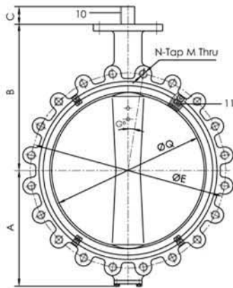
Front View VBFLY-DL1 Lug Ductile Iron
