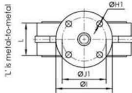
Front View VBFLY-DL1 Lug Ductile Iron
