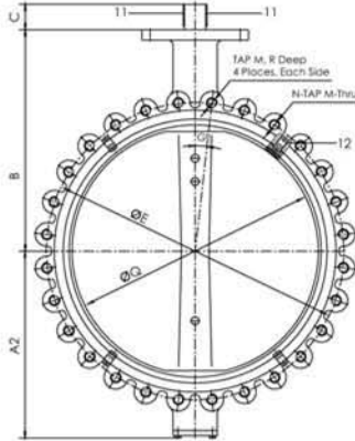
Front View VBFLY-DL1 Lug Ductile Iron
