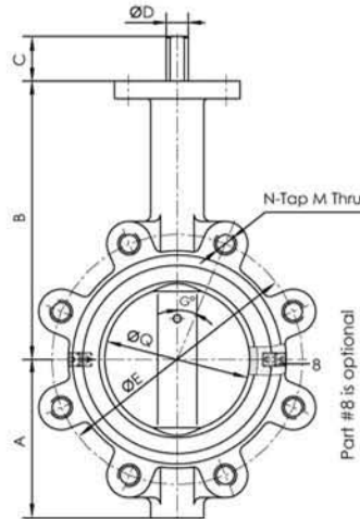
Front View VBFLY-DL1 Lug Ductile Iron
