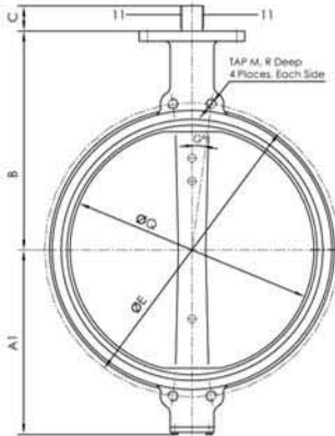
Front View VBFLY-IW1 Wafer Cast Iron
