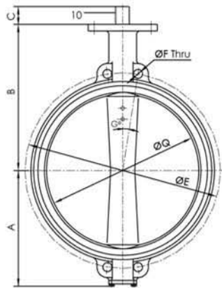
Front View VBFLY-IW1 Wafer Cast Iron
