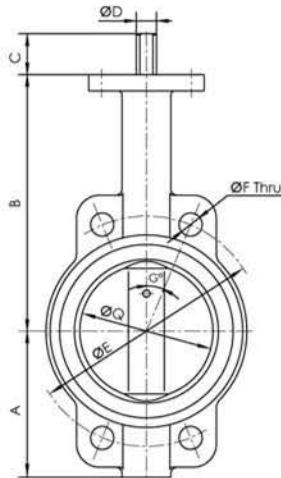
Front View VBFLY-IW1 Wafer Cast Iron
